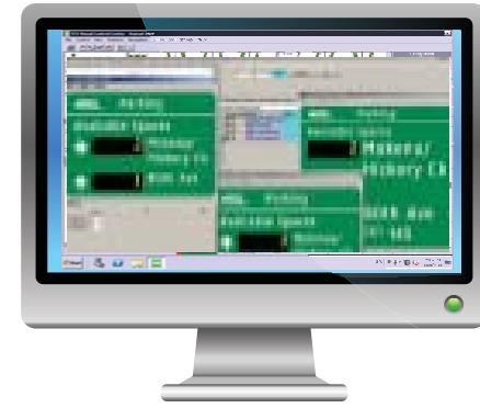
PGS SOFTWARE
